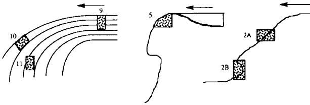
Figure 4. The location of the tufa samples: diagrammatic downstream profiles of three tufa dams indicating the relative positions from which the tufa samples were cut (numbered blocks). Left, gentle slope as in Fig 2b; middle, lip overgrowth as in Fig 2c.
