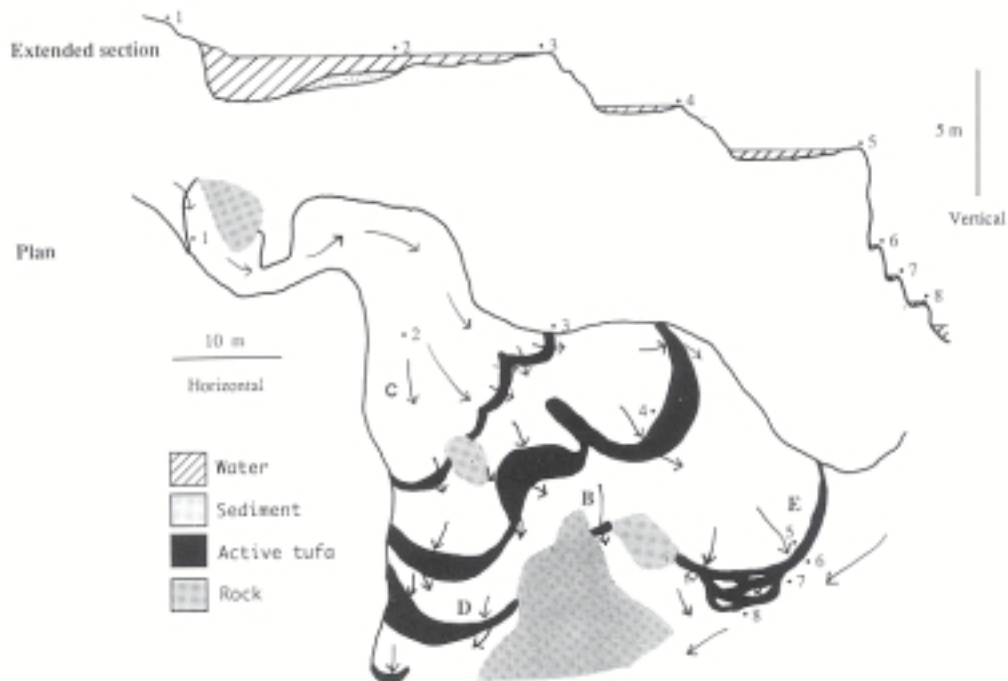
Figure 3. Plan and extended section of the tufa deposit below Og Cave with the apparently active tufa faces shown in black. The stream emerges from Og Cave (1) and spreads through a series of pools formed by tufa dams (3-8), before the confluence with another stream below the final dam (8). Some tufa dams have a narrow sill and a nearly vertical downstream face from which the water falls (3, 5-8; see Fig 2c), while others have a broad sloping sill over which the water has a riffle flow (4, D see Fig 2b). Main dam (5); B marks the site of the sill referred to in the text; dam of the upper pool (3); D denotes sites from which tufa samples were collected; E marks the approximate site of the fracture in the lower tufa dam caused by an earthquake in 1972.
