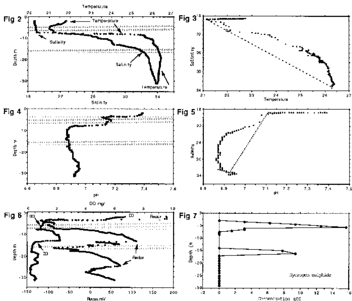
Figure 2. Profiles of Bundera Sinkhole in 1997 where the grey bands denote the zones of elevated hydrogen sulphide concentration (see Fig 3F), the descent rate was 0.05 m s -1 (sd 0.028, n=21). A; Temperature (°C) and salinity (g L -1 TDS) profiles. B; the salinity-temperature relationship of the vertical profiles where the dotted line denotes the conservative mixing hypothesis. C; pH profile. D; the salinity-pH relationship of the vertical profiles where the dotted line denotes the conservative mixing hypothesis. E; dissolved oxygen (mg L -1 DO) and oxidation reduction (redox) potential (mV) profiles. F; the vertical distribution of H 2 S (as total acid soluble sulphides, μM).
