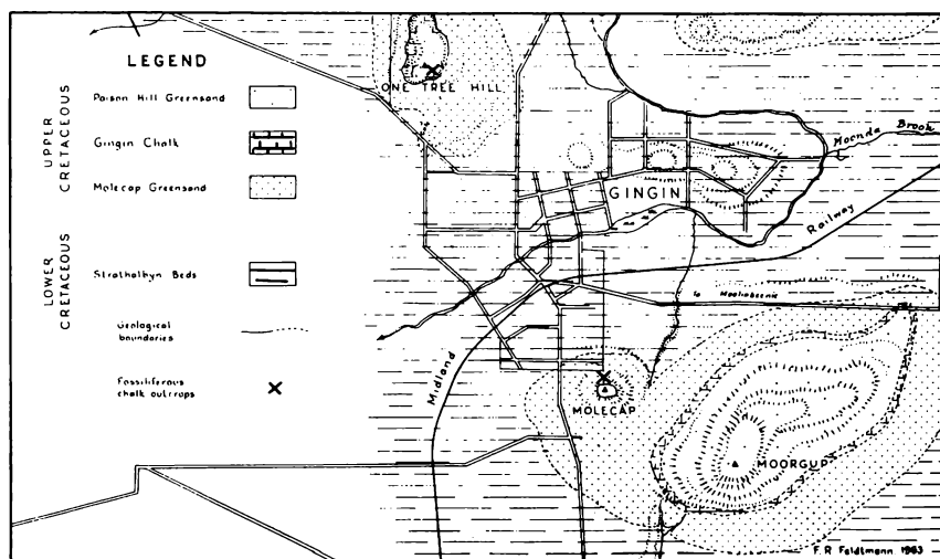
Geological map of the Gingin region (from Feldtmann 1963)
